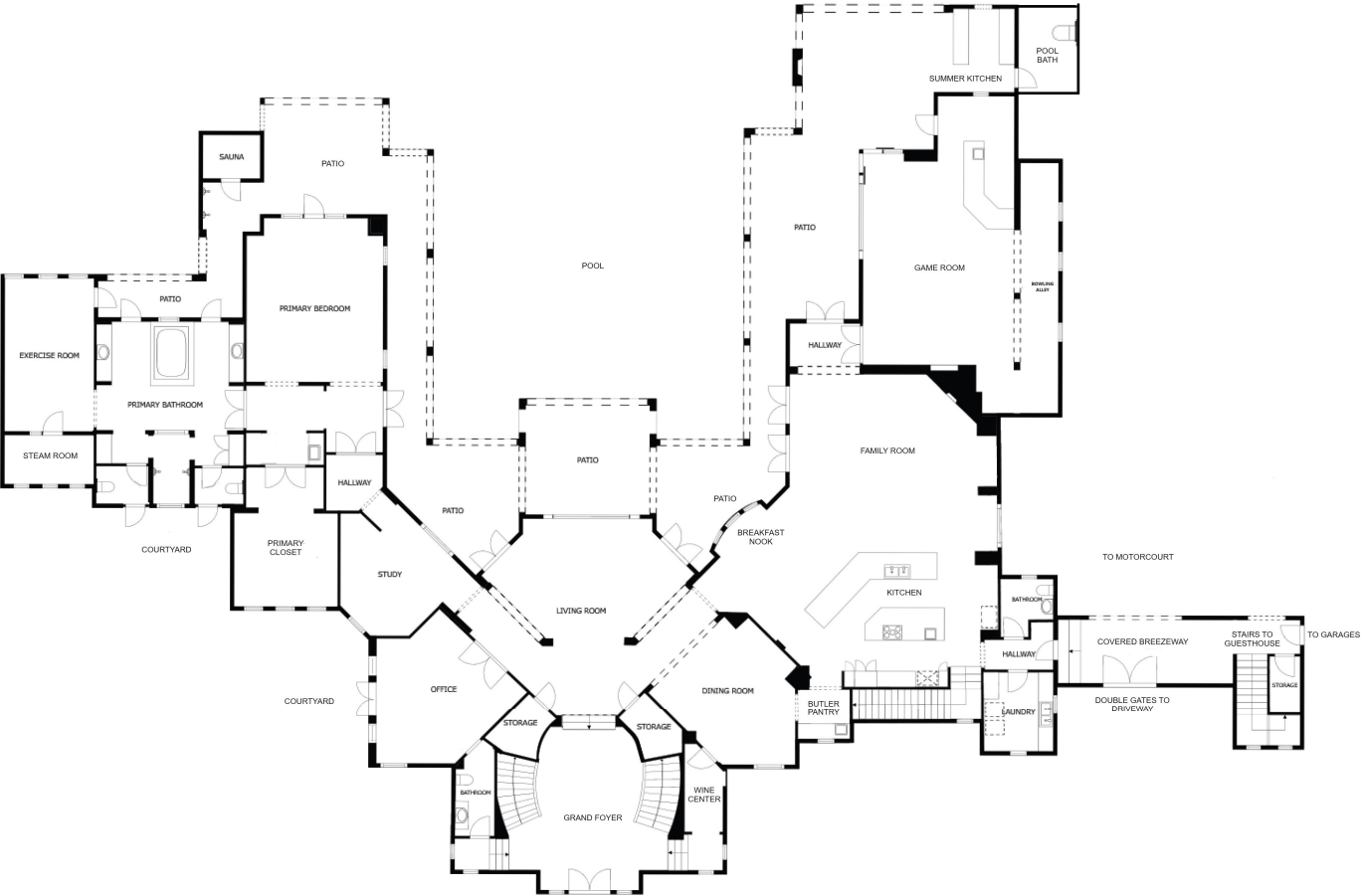
FLOOR 1
